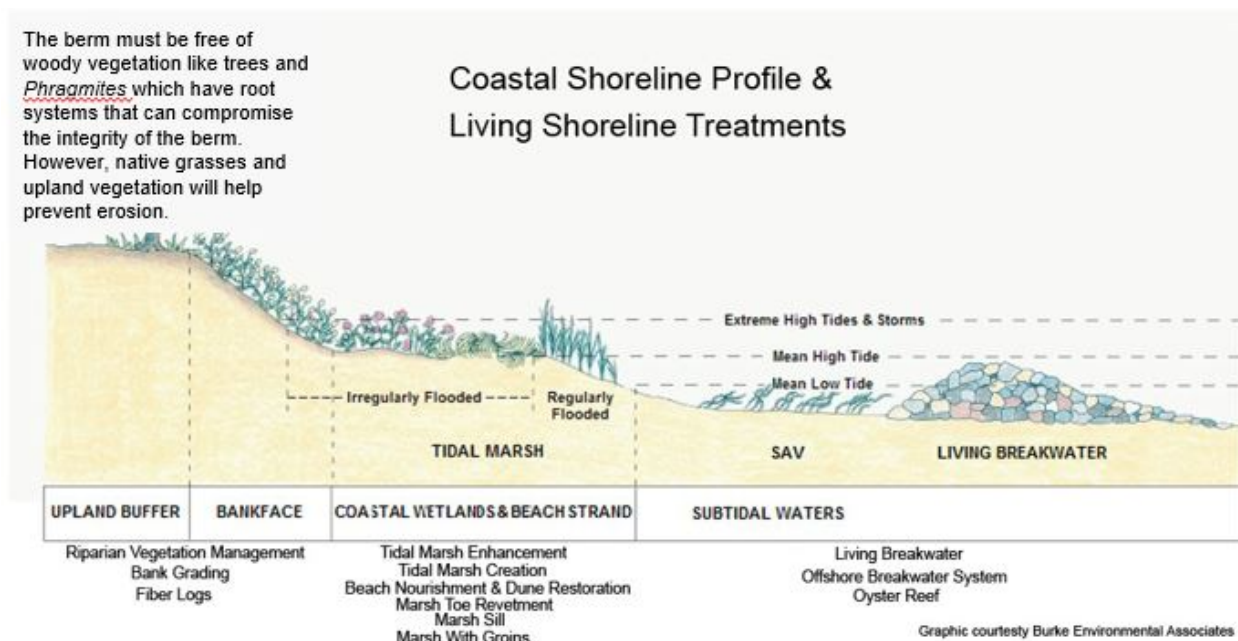
Figure 5-10: Profile drawing of an NNBFF, or living shoreline, concept
